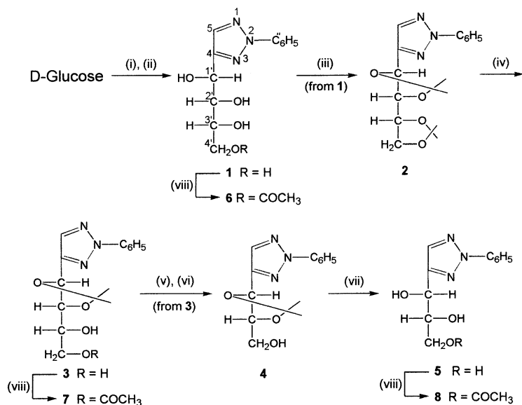
Scheme 1. Reagents and conditions: (i) PhNHNH 2 , acetic acid, H 2 O, reflux; (iii) 1% aq CuSO 4 •5H 2 O solution, H 2 O, reflux; (iii) FeCl 3 , acetone, stirring, 25–28 °C; (iv) 80% acetic acid, stirring, 25–28 °C; (v) NaIO 4 , H 2 O/dioxane (1:1), stirring, 25–28 °C; (vi) NaBH 4 , H 2 O/dioxane (1:1) ethanol, stirring, 25–28 °C; (vii) 80% acetic acid, reflux; (viii) CAL-DIPE/PPL-THF, vinyl acetate, 42–45 °C.
